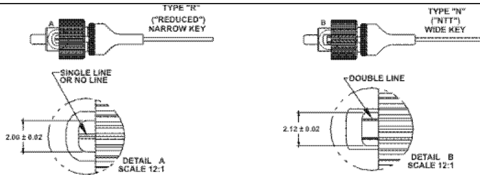
Figure 5. Narrow Key Versus Wide Key Connectors
