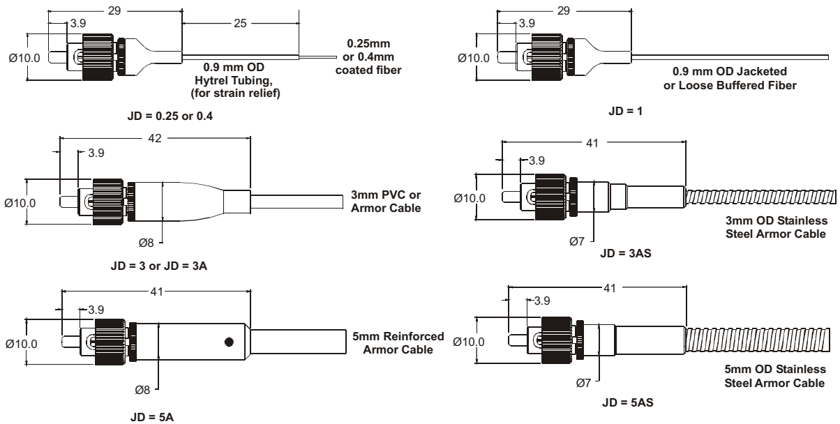
Figure 4. PM FC Connector Dimensions for Various Cable Sizes
