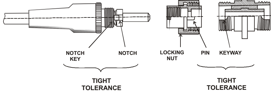
Figure 2. PM FC Connector Construction
