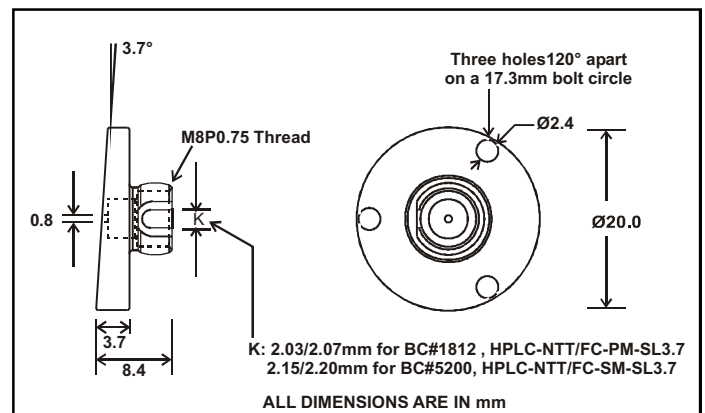
Figure 7. Bulkhead Angled FC Receptacle
