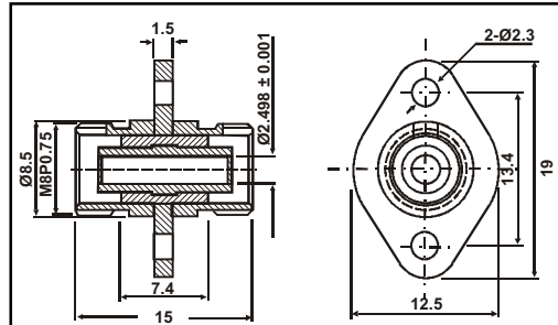
ALL DIMENSIONS ARE IN mm. Figure 3. FC Sleeve Thru Connector Dimensions
