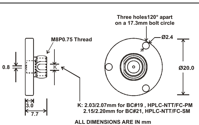
Figure 6. Bulkhead FC/PC Receptacle
