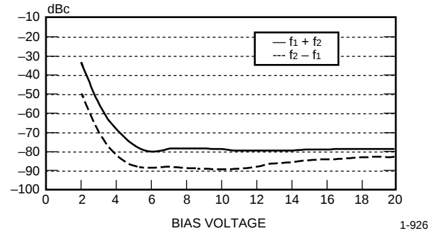
Figure 7. Second-Order Linearity, 1310 nm Wavelength; 0 dBm Optical Received Power; Two Tones @ 35% OMD per Tone
