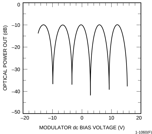
Figure 5. Output Power vs. Bias Voltage
