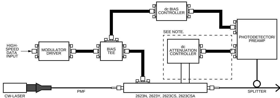
Figure 1. Recommended Operating Circuit Diagram
